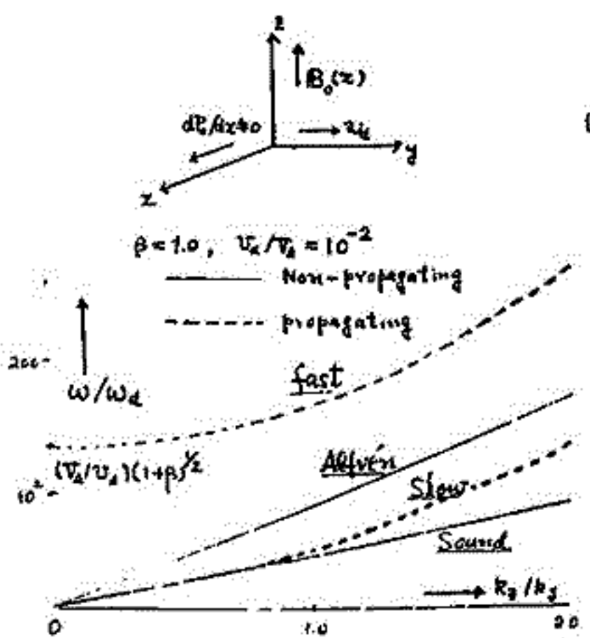
Fig. a HN-WAVES (non-drift modes)
