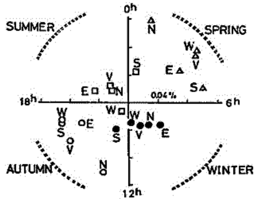
SEASONAL VARIATION OF FIELD DEPENDENT SOLAR DIURNAL VECTORS (MISATO)
