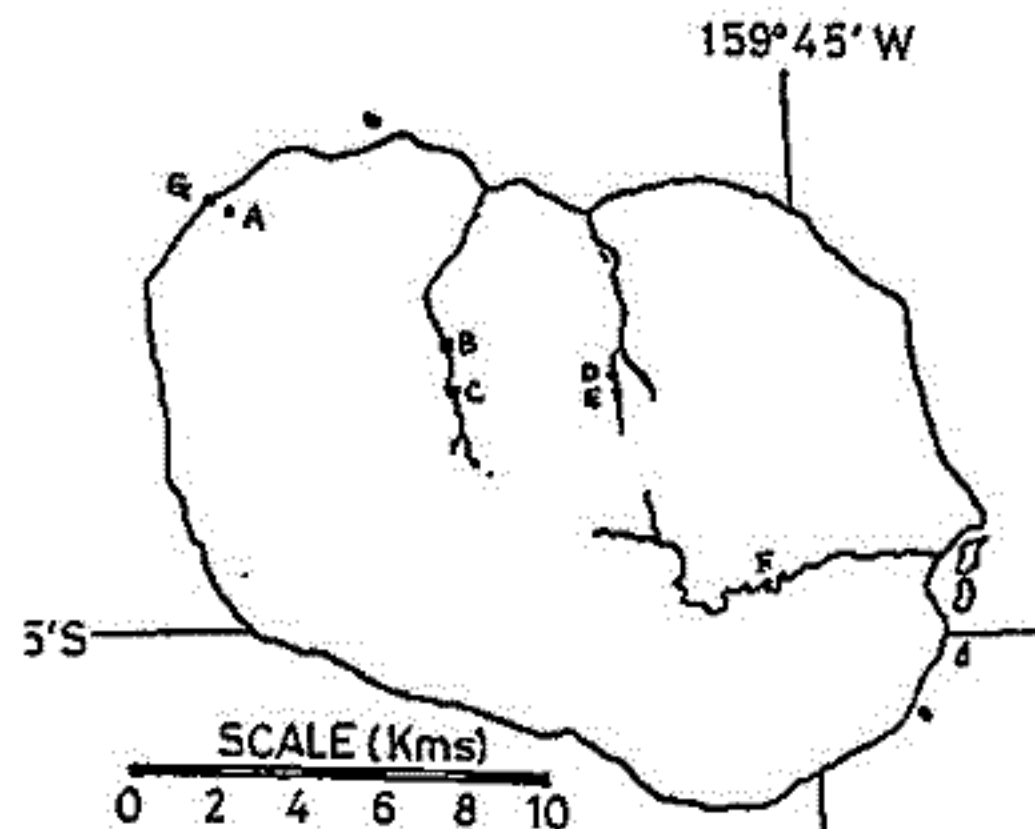
Fig.1 RAROTONGA island Sampling localities
