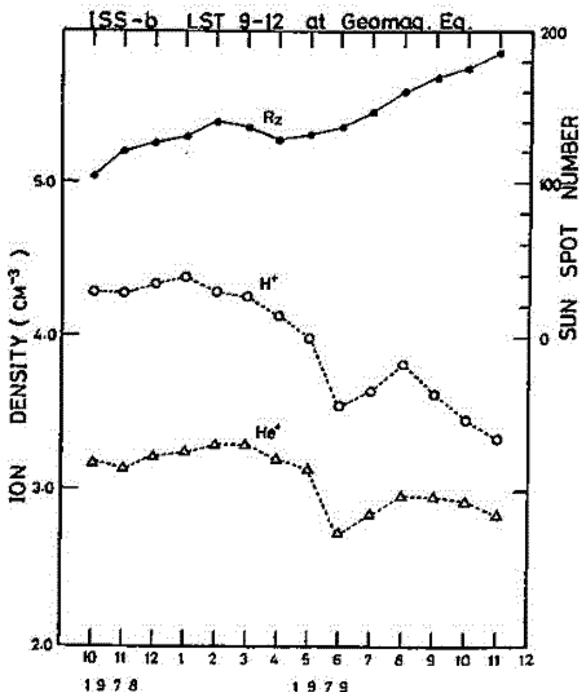
Variation of H + , He + and R z with 4-month Moving Average
