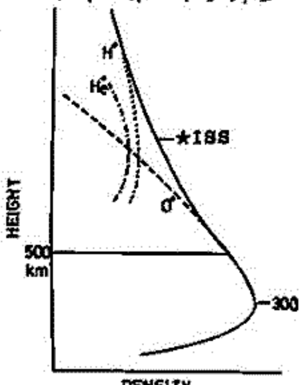
Fig. 1. Ionospheric profile.
