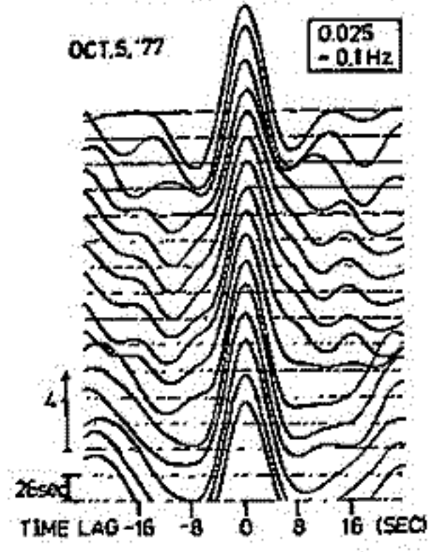
図3 0.025~0.1 Hz の強度変動の dynamic cross-correlation
