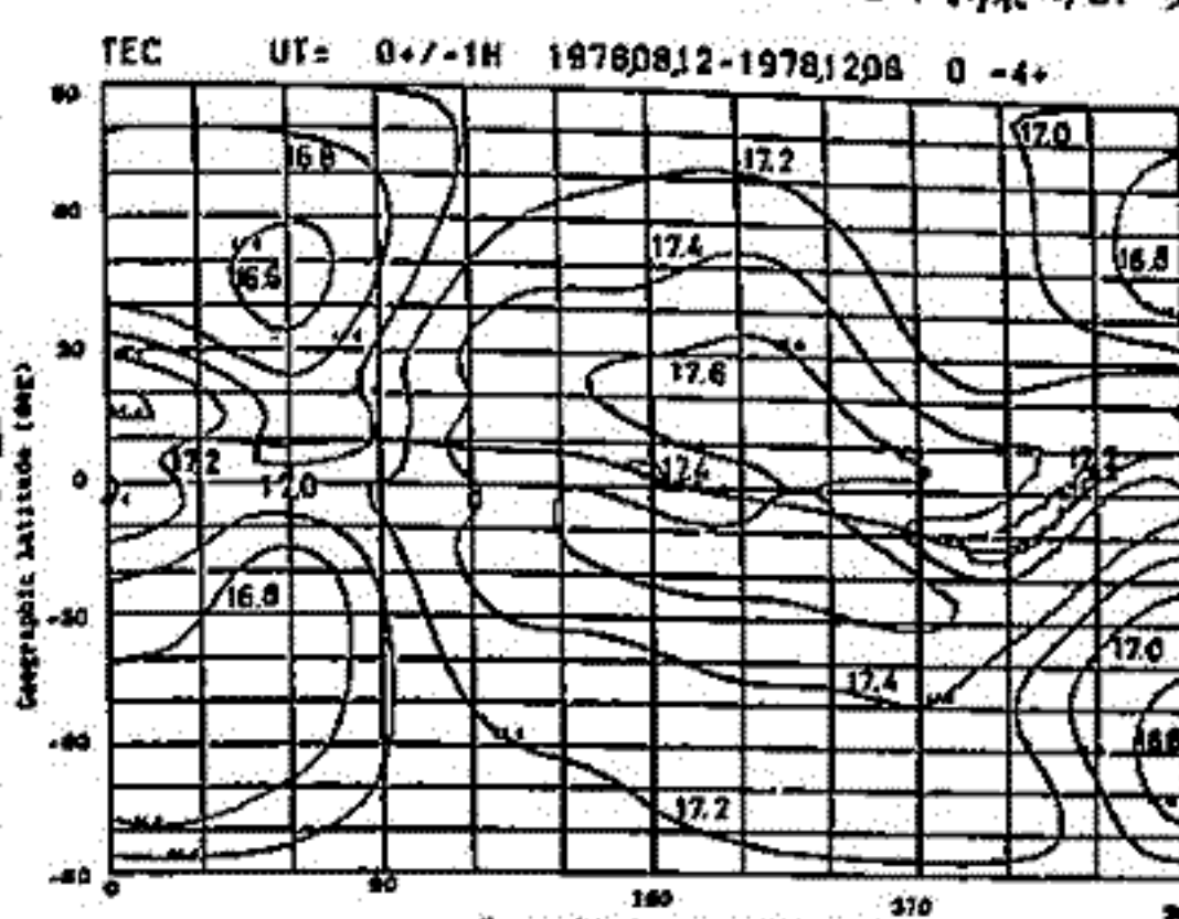
Fig. 2. Ionospheric total electron content contour man by Diffusive eq. & Alpha-Chapman's eq.
