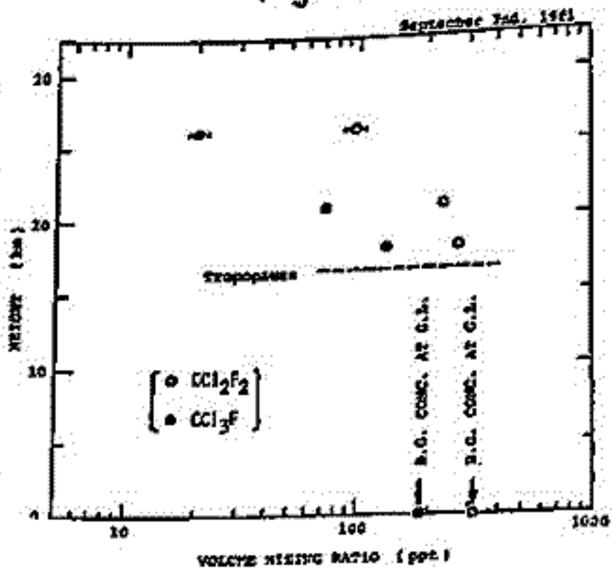
Fig. 3 Vertical Distribution of CCl_2F_2 and CCl_3F .
