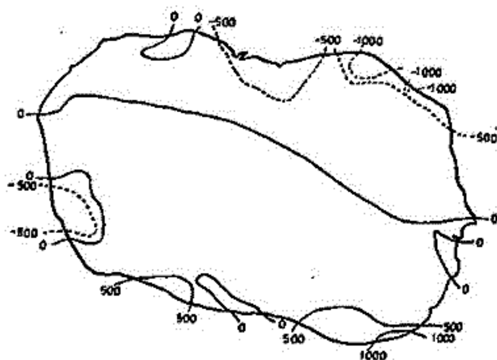
Fig.2 observed anomaly (unit;nT) (observed value-IGRF)
