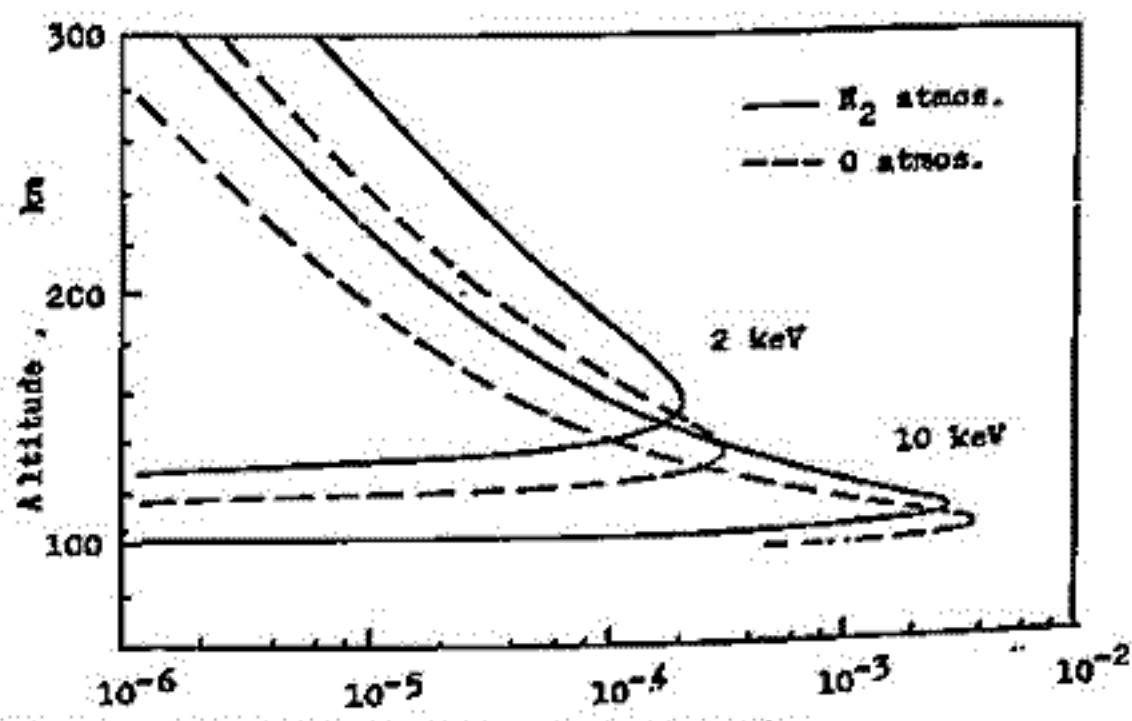
Fig.1 Normalized Energy Deposition Rate, (eV/cm 3 sec)/(electron/cm 2 sec)
