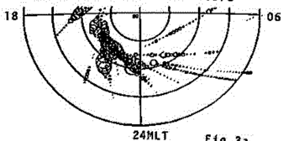
AURORAL HISS INTENSITY (ISIS) WINTER (MAY-JULY) 1976-1978
