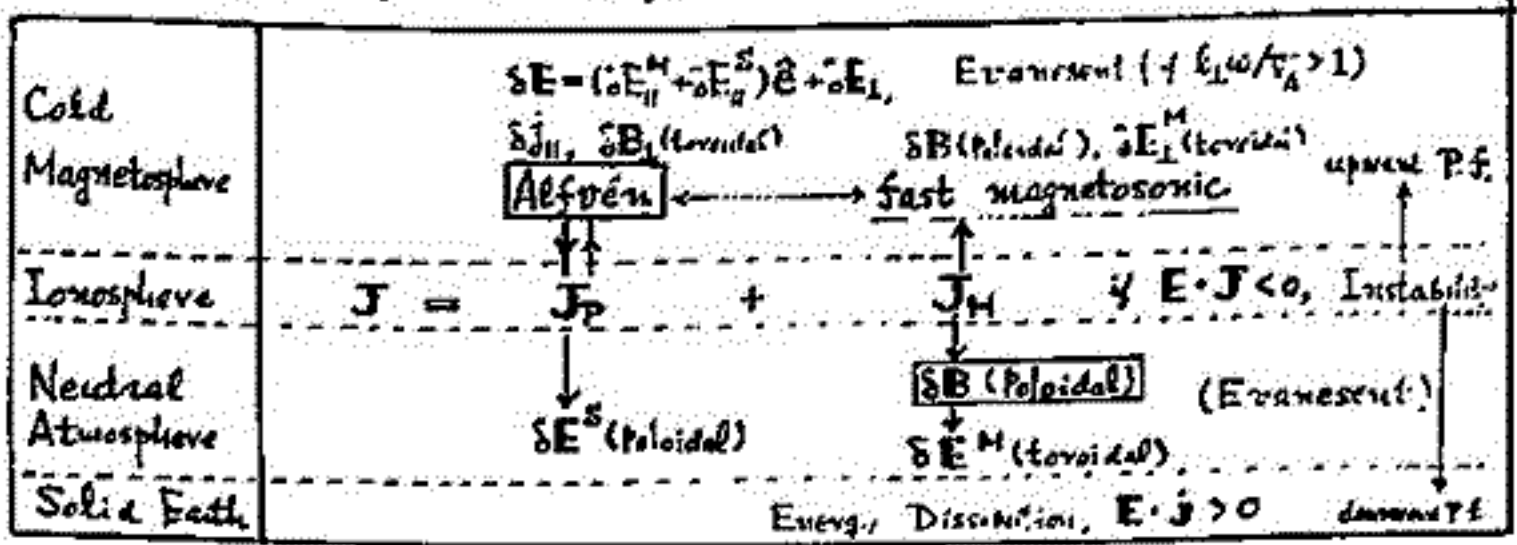
(a) Incidence of Shear Alfvén Wave
