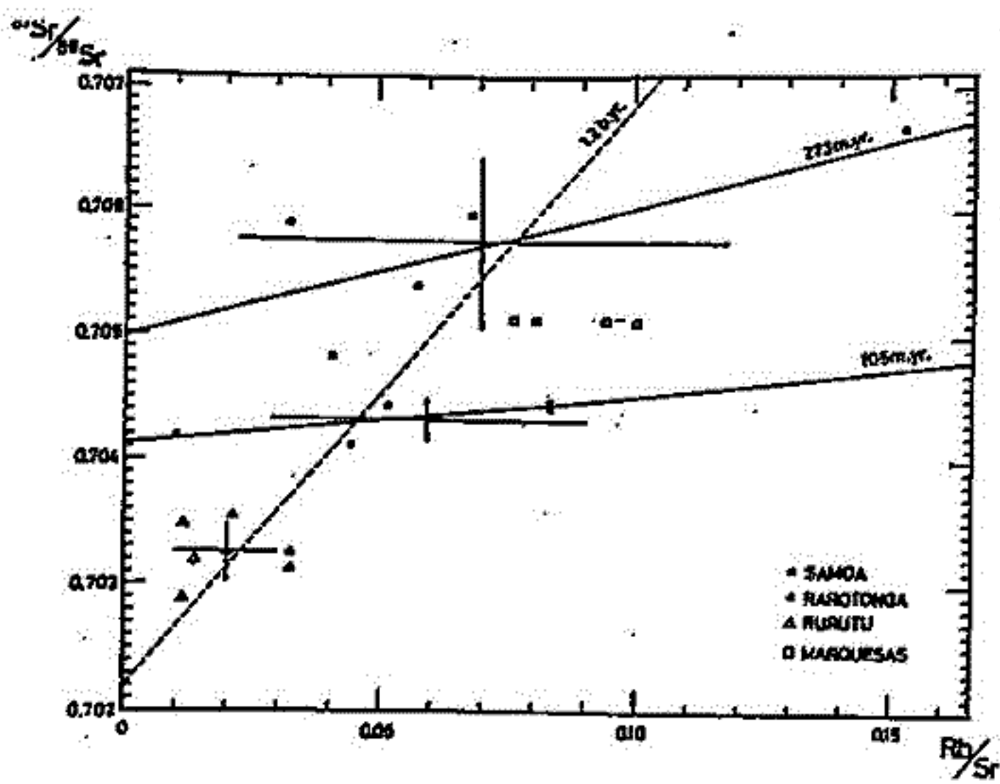
Rb/Sr — ( 87 Sr/ 86 Sr) diagram for the samples from Samoa, Rarotonga, Rurutu and Marquesas. The points with error bars are average points for individual islands. The dotted line is the isochron for the three average points. Two lines are isochrons for Samoa and Rarotonga.
