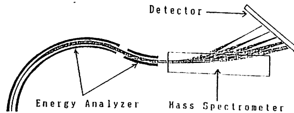
Fig. 1 Ion trajectories in the IMS consisting of the tandem energy analyzer and orange mass spectrometer
