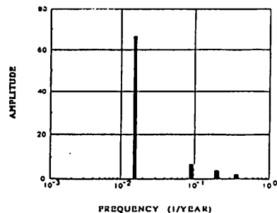
Fig.3 The spectrum obtained by Sompi method
