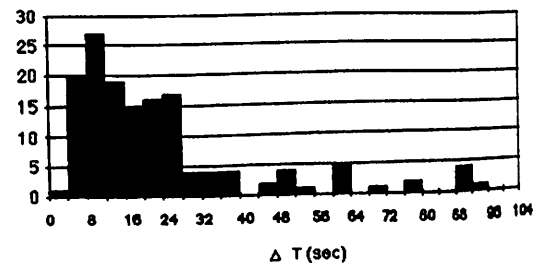
Fig.2. Histogram for the time interval of repeating bursts.
