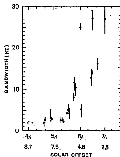
Fig.2 Radial dependence of spectral broadening
