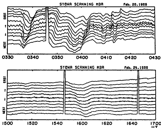
Fig.1 Auroral absorptions drifting eastward in the morning sector (upper panel) and westward in the afternoon sector (lower panel), observed with the scanning-beam riometer.
