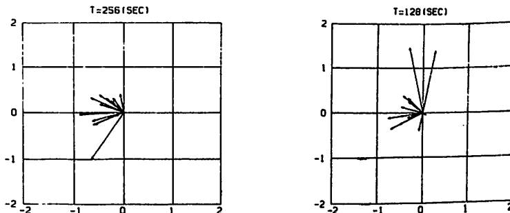
Figure 1 Induction vectors calculated for SC's and SI's without substorm from 1981 to 1984. Upward is geophysical northward.
