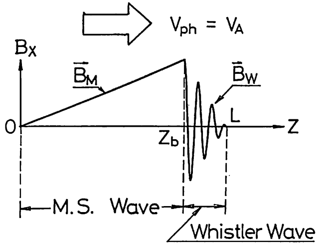
Fig. 1 Model cometary waves used in the test particle simulation
