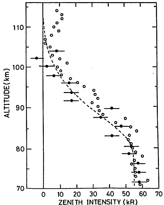
Deduced O 2 1.27 μm nightglow emission profiles. Present observation is represented by the solid circles. The results obtained by Evans et al. (open circles) and by Thomas and Young (broken curve) are also shown.
