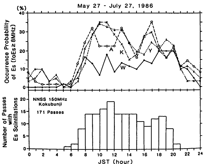
Fig. 2. Diurnal variations of the number of satellite passes accompanied by Es scintillations (bottom) and the occurrence probabilities of foEs ( \geq 8 MHz) at four ionosonde stations (top).
