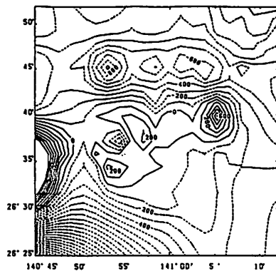
Fig. 2 Total intensity anomaly map around the Kaikata Seamount. Contour interval is 100nT.
