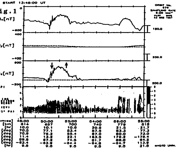
DE-2 MAG DAY261 8 SEP 1981 SPC
