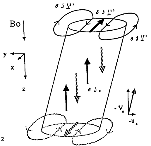
Fig. 2 V_A Alfvén Velocity u_0 Io's Velocity
