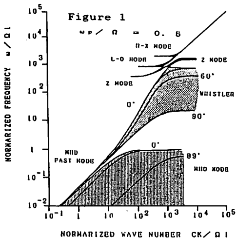
Figure 1. \omega - k diagram in the wide range of frequency, from MHD mode waves to free space mode waves.
