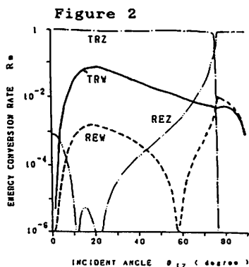
Figure 2. Energy conversion rate form Z-mode wave to whistler mode wave.
