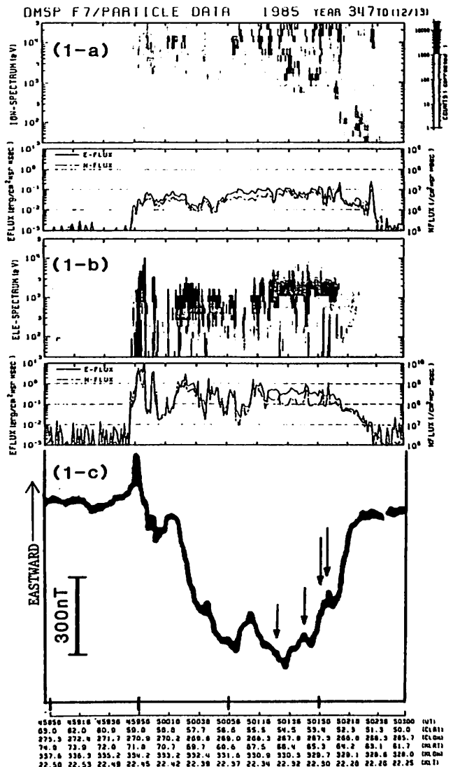
Fig.1. Summary plots of precipitating ions(1-a), electrons(1-b), and magnetic Bz(east-west) component(1-c) observed on DMSP-F7 at 04:59 - 05:03 UT on December 13,1985. Four arrows in (1-c) correspond to LEEP events in (1-b).
