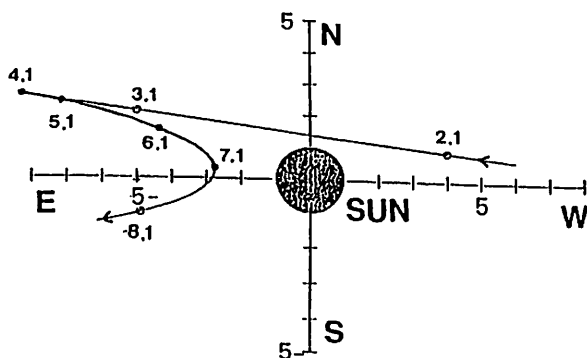
Fig.1 'SAKIGAKE' trajectory seen from the earth
