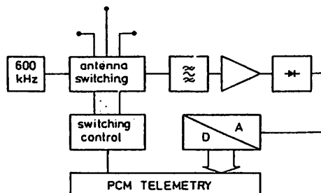
Fig.2 Schematic of the instrument.
