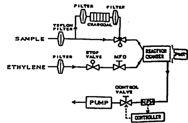
Fig. 1 Schematic diagram of the ozone instrument. (MFC: Mass Flow Controller, MFM: Mass Flow Meter, PMT: Photomultiplier Tube)
