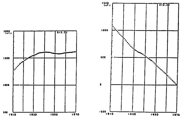
Fig.1 Time variation of Gauss coefficient g_2^2 h_2^2
