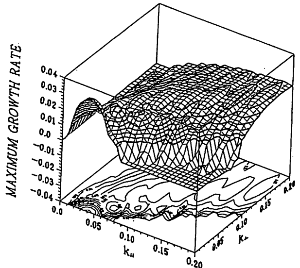
Fig. 1: The three dimensional display of the maximum growth rates. The axis of k_{\parallel} ( k_{\perp} ) represents the wave number in the direction of the ambient magnetic field(perpendicular direction).
