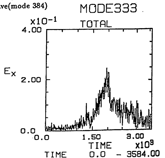
Fig.3: The k-spectra evolution of bernstein wave(mode 333)
