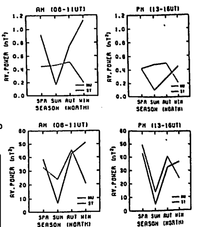
Fig. 3 Seasonal variation of Pc5 (upper) and Pc3 (lower) pulsation power averaged at morning side (left) and at afternoon side (right).
