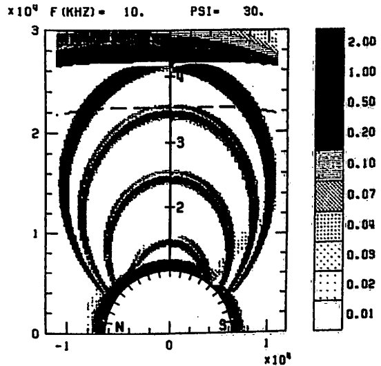
Fig. 2. 3 ducts ( L=1.5, 2.5 and 3.5 ) are displayed on the gray scale to indicate the guiding strength at the both edges of duct in the condition of enhancement factor = 0.5, duct width = 0.5(L) , \psi=30^\circ and f=10\text{kHz} .
