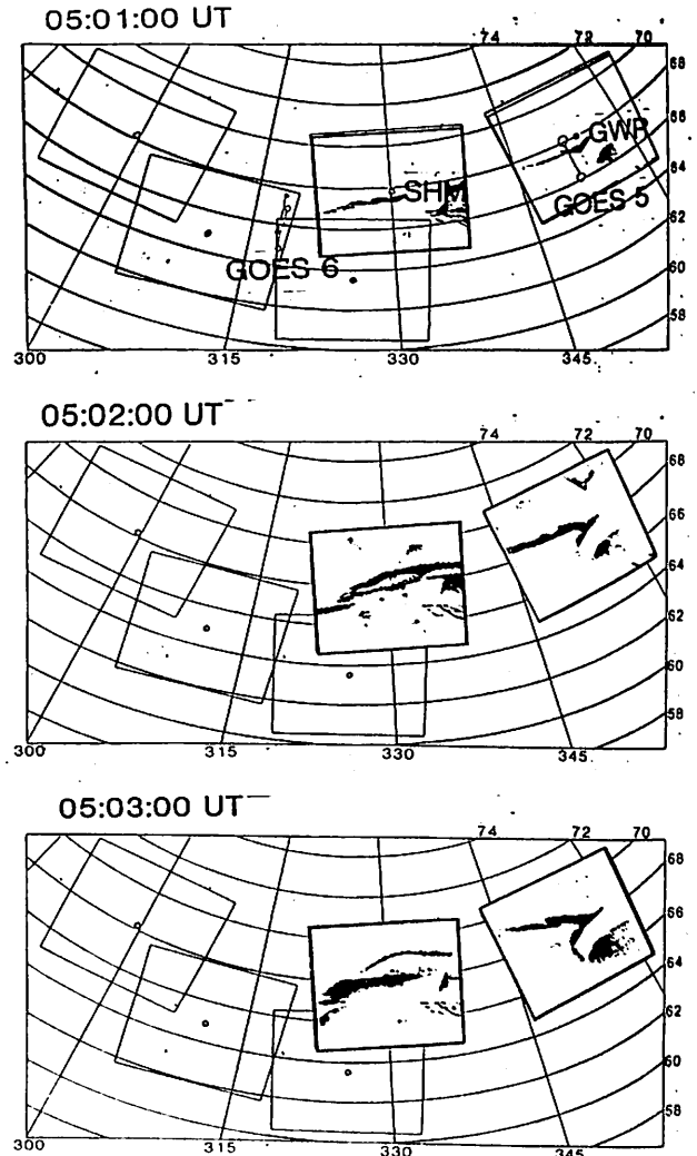
Fig. Sequential Pictures of Auroral expansion at 05:01 UT, Jan. 27, 1986.
