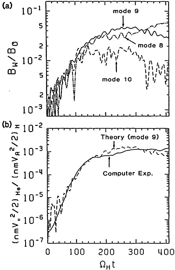
Fig. 1. (a) Time history of the dominant modes (mode 8, 9 and 10). (b) Time evolution of the helium energy density in the parallel direction. The solid line represents the simulation result. The dashed line is the theoretical value computed from the wave amplitude of mode 9.
