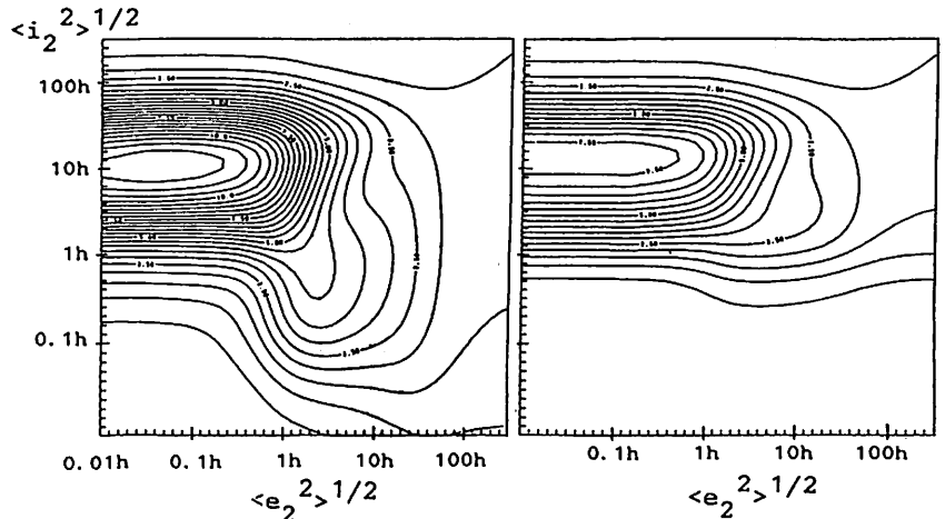
Fig. 2 Total Collisional Rate e_1 = i_1 = 0
