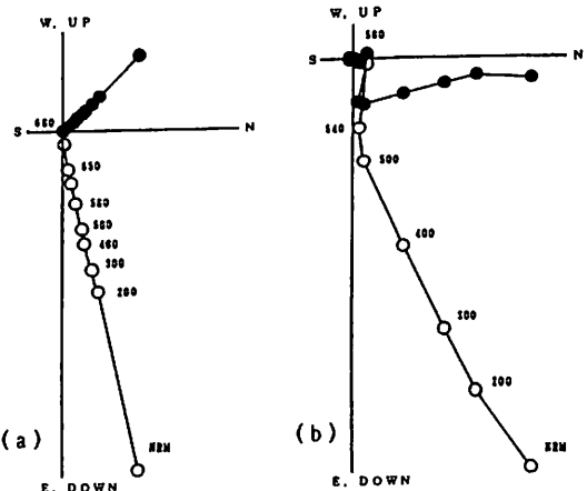
Fig.2 Examples of stepwise thermal demagnetization before tilt correction
