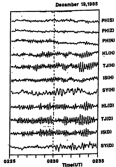
Fig 1 : Wave form of pulsating aurora at Husafell, the H and D component of magnetic pulsations at Husafell, Tjornes, Isafjordur in Iceland and at Syowa Station in Antarctica.
