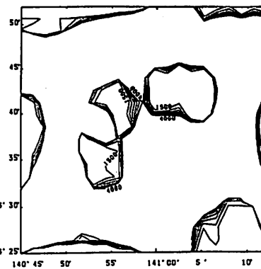
Fig. 3 Depth contours of the igneous rocks of which magnetic moment is 0.7\text{Am}^2 . Contour interval is 500m.
