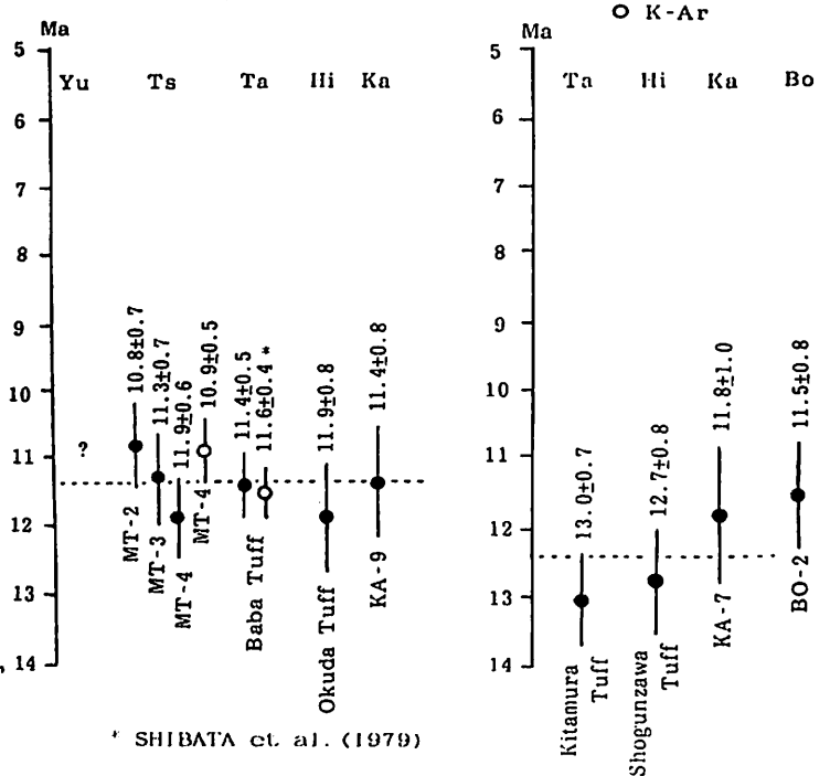
Radiometric ages of Miocene tuffs.
