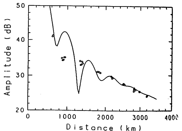
Fig.2 Computed field strength versus distance (solid curve) using our wave guide mode method in comparison with those measured (data No. III) in the daytime(2:00 - 6:00 U.T.).
