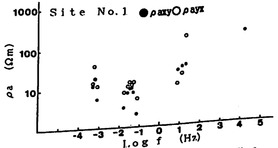
Fig.2 Apparent resistivity against frequency at No.1.
