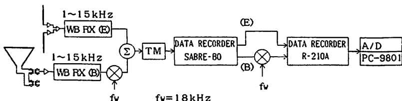
Fig.1 Block diagrams of wide band receiver and data analysis
